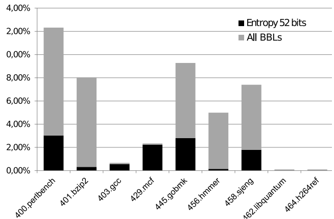
Figure 9: Runtime Measurements with SPEC CPUint2006
