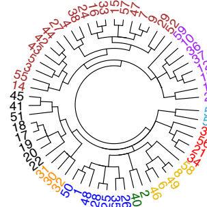
(f) K = 9
