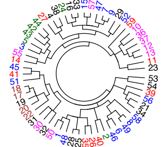
(g) Autonomy
