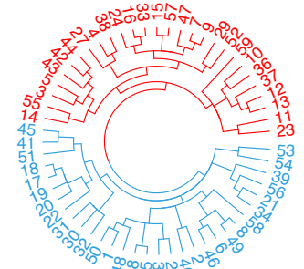
(c) K = 2
