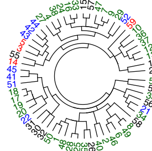
(f) K = 9
