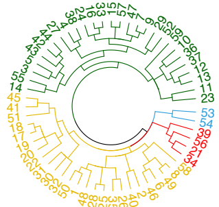
(e) K = 4
