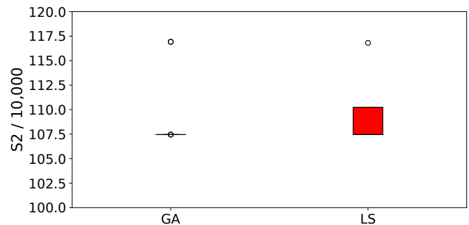
Fig. 18: Boxplot of the tour length score ( S_2 ) to be minimized for the TSP-PD problem instance for all algorithms
