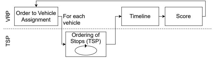
Fig. 2: Overview of the two-staged strategy.
