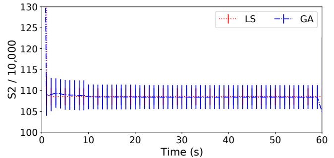
Fig. 17: Mean and standard deviations of tour length score ( S_2 ) to be minimized for the TSP-PD problem instance for all algorithms.
