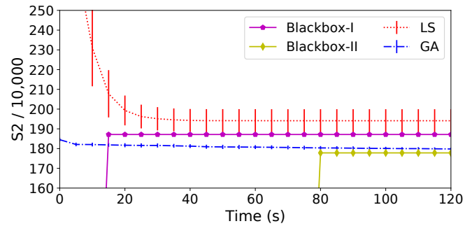
Fig. 13: Mean and standard deviations of tour length score ( S_2 ) to be minimized for the VRP-I-P problem instance for all algorithms.
