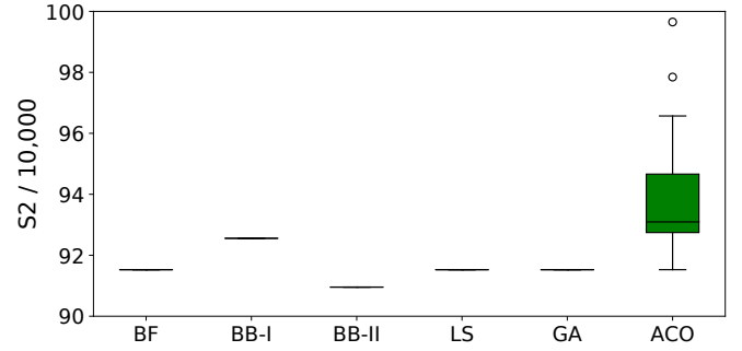
Fig. 6: Boxplot of the tour length score ( S_2 ) to be minimized for the TSP-I problem instance for all algorithms.
