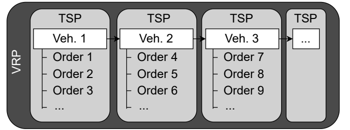
Fig. 3: Illustration of an object-oriented genome representation of the GA.
