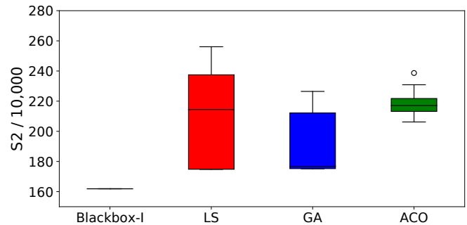
Fig. 10: Boxplot of the tour length score ( S_2 ) to be minimized for the TSP-II-P problem instance for all algorithms.
