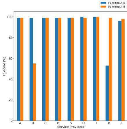
Fig. 13: Generalization check of the FL model: Service Providers B and K are not involved in federated training process.
