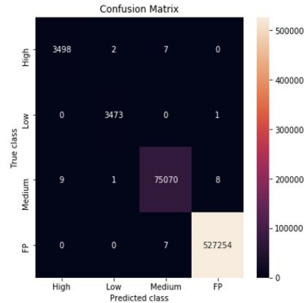
Fig. 10: Confusion matrix of model G on local test data
