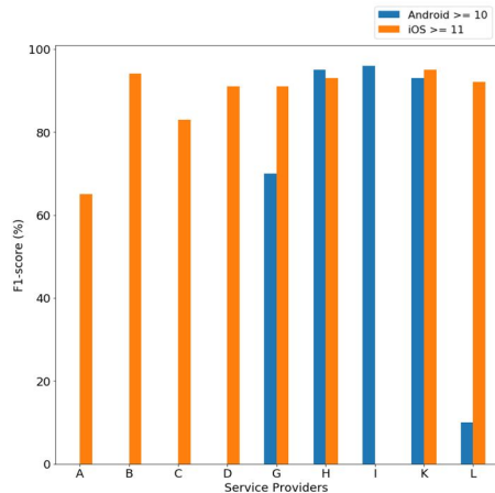
Fig. 14: Generalization check of the FL model. Android OS above 9 and iOS above 10 are not involved in federated training process.
