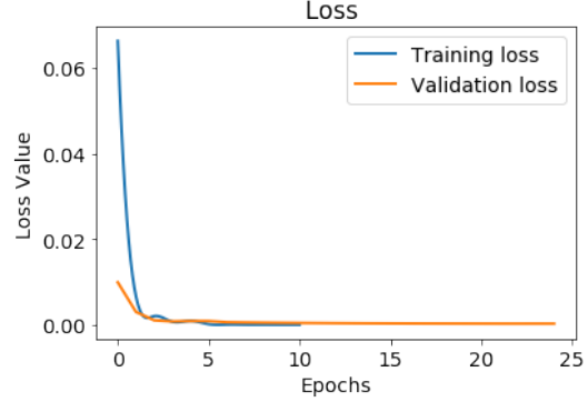
Fig. 8: Learning curve: training and validation loss
