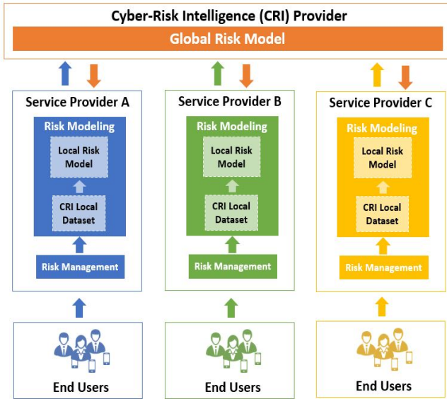
Fig. 1: High-level overview of FedCRI platform
