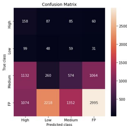
Fig. 11: The CM of the model G on test data of Service Provider C
