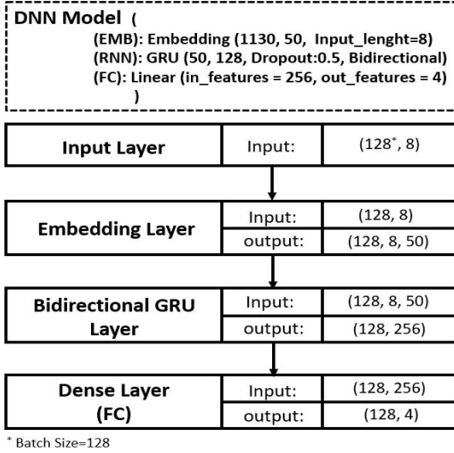
Fig. 4: DNN Classifier Architecture.
