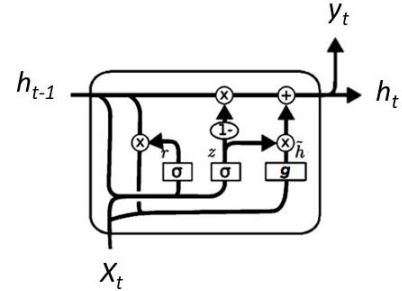
Fig. 15: GRU gating mechanism
